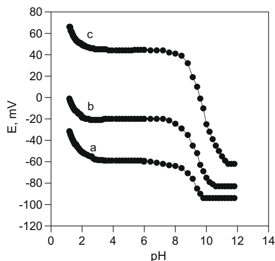
Figure 3 Effect of the test solution on the potential response of the PPAFM electrode (a) 1 \times 10^{-4} , (b) 1 \times 10^{-3} and (c) 1 \times 10^{-2} .
