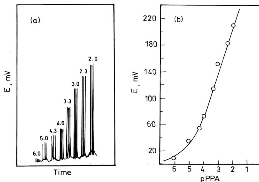
Figure 2 Recording (a) and its corresponding calibration graph (b) for PPA-PM electrode under FI conditions.
